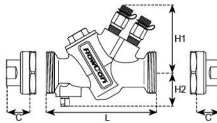
FlowCon ABV with composite cartridge
