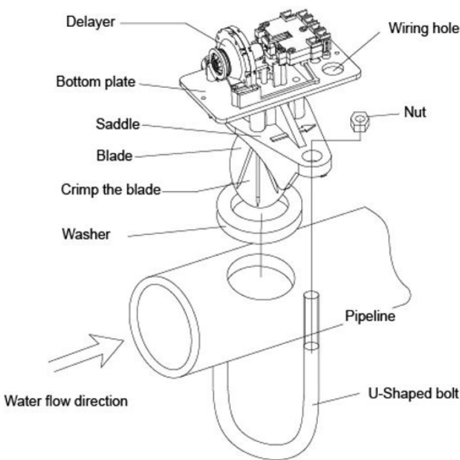
Figure 2 Installation Drawing
