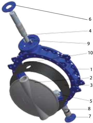
DN700-1200
