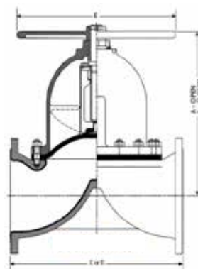
Flanged DN200-DN350
