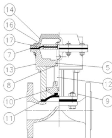
Double Acting
