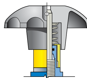
Sealed Bonnet In cases where hazardous liquids or gases are being handled and where additional safety features are considered to be necessary.
