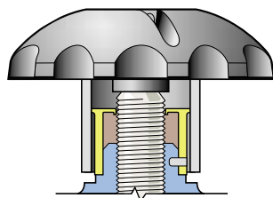
Lubrication Bonnet assembly lubricated for life. Needs no additional grease. The indicator lip seal stops the ingress of dust, dirt and atmospheric contaminants.
